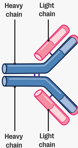
Immunoglobulin structure
